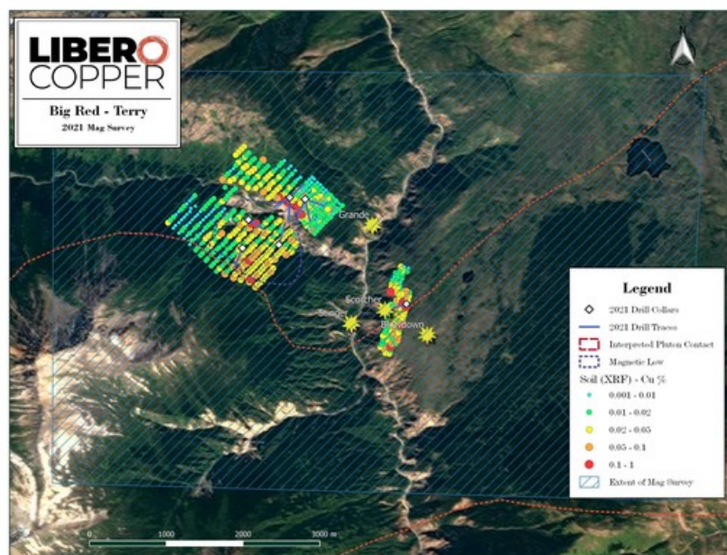
Figure 1: Plan map illustrating the coverage of the new magnetic survey, pXRF soil sample results and the 2021 drill program on and around the Terry Target. (CNW Group/Libero Copper & Gold Corporation.)
