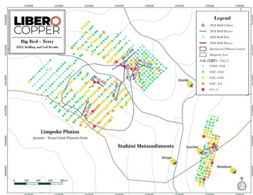
Figure 3: Plan map illustrating the distribution of drilling at the Terry target and the XRF Cu-in-soil results from the soil sampling programs. (CNW Group/Libero Copper & Gold Corporation.)
